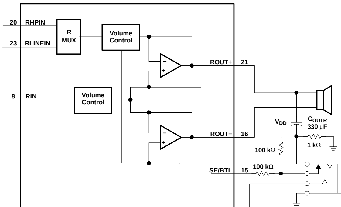
Figure 47. TPA0222 Resistor Divider Network Circuit
