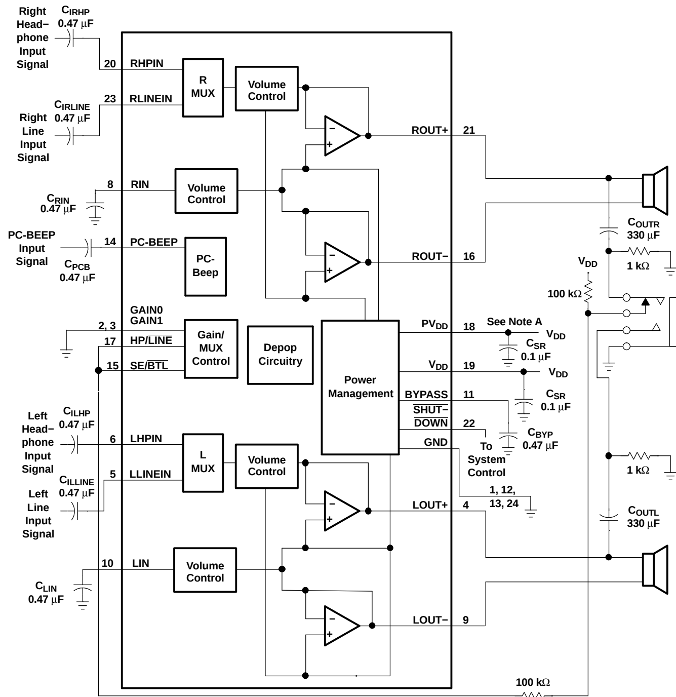
Figure 42. Typical TPA0222 Application Circuit Using Single-Ended Inputs and Input MUX
